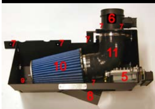
7. Fit the 6 plastic clip to the OptiFlow heat shield (7). And the external intake shield (8). Assemble the ECU (5) the air mass meter (6) the air filter rod (9) the air filter (10) and the inlet hose (11).
